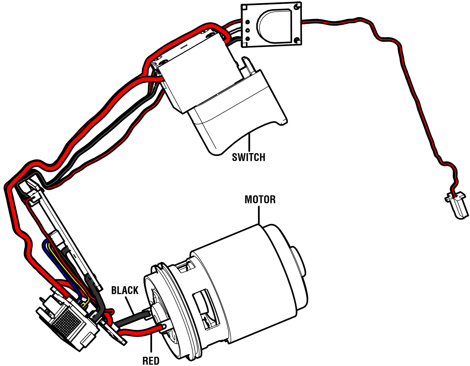
WIRING DIAGRAM
