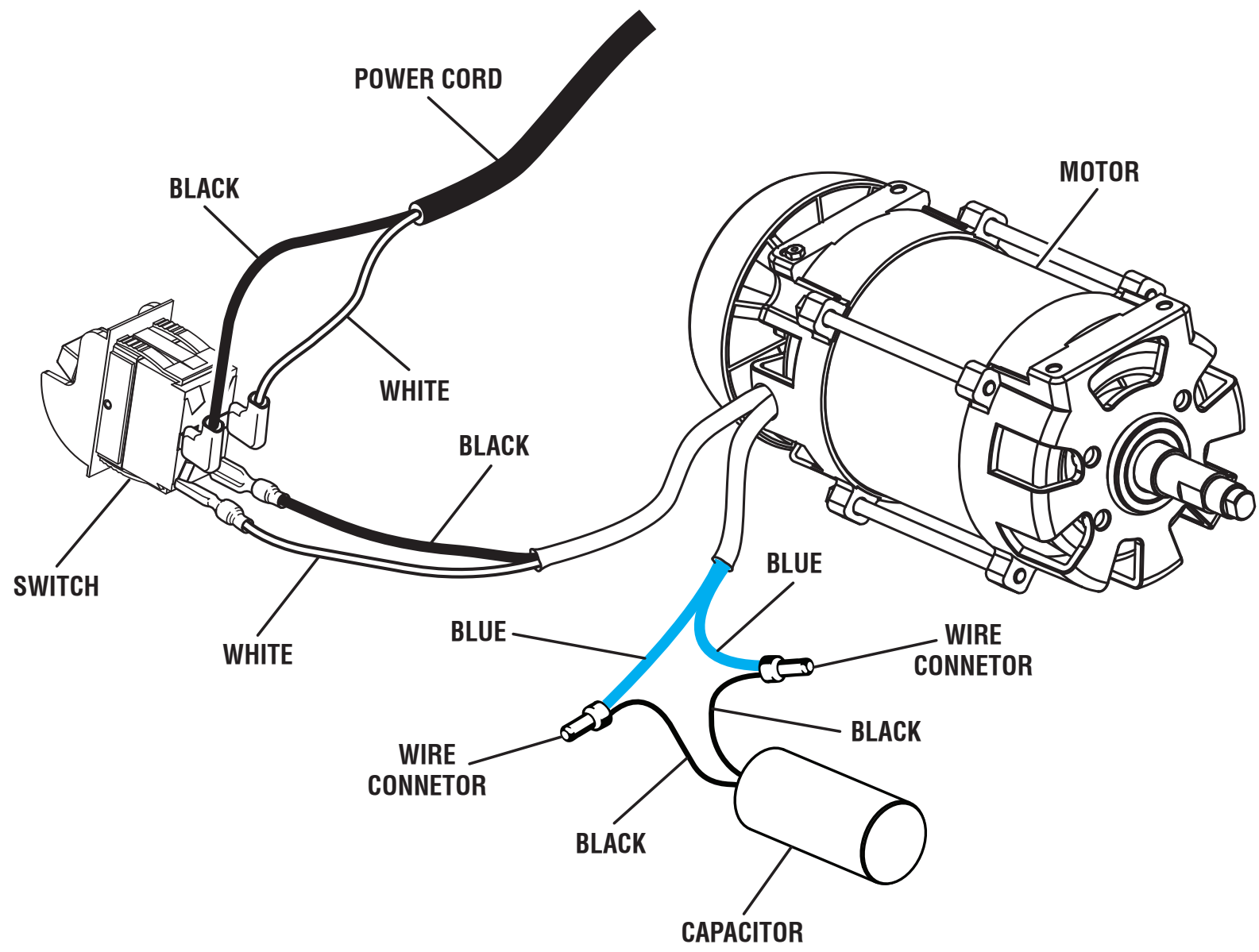
WIRING DIAGRAM
