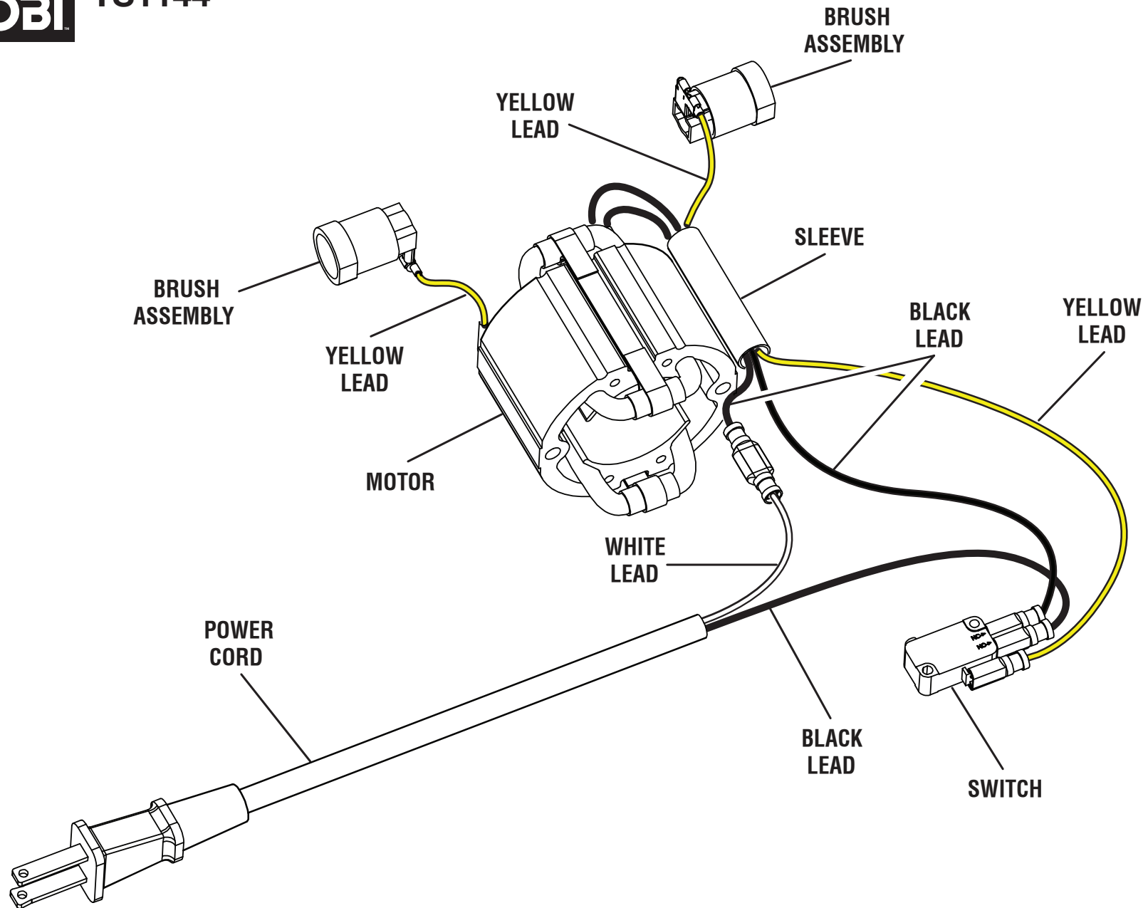
WIRING DIAGRAM
