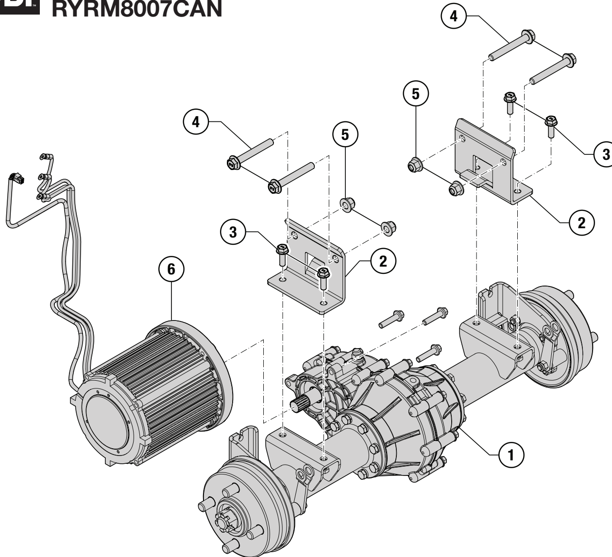
PARTS LIST — FIGURE I
