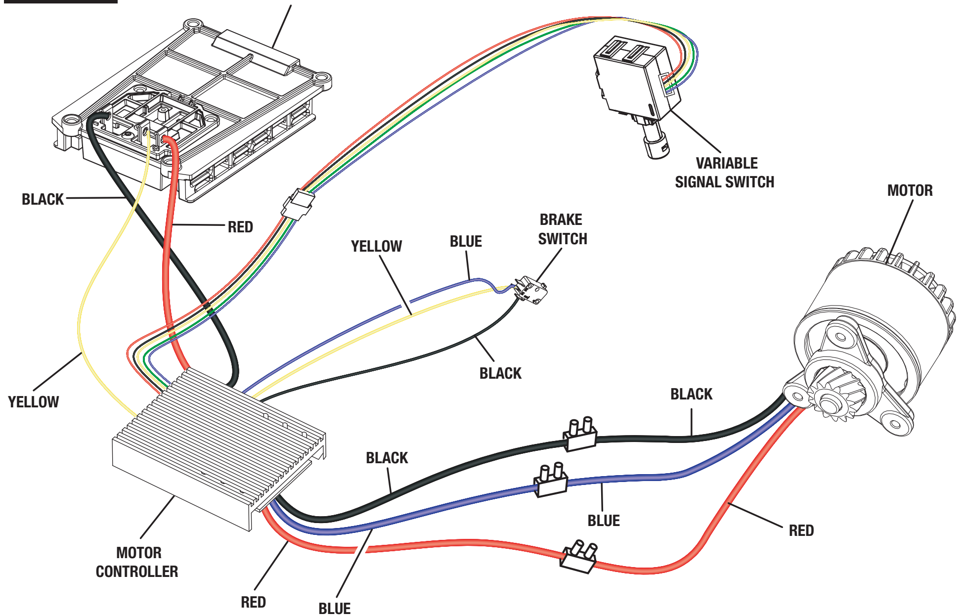
WIRING DIAGRAM
