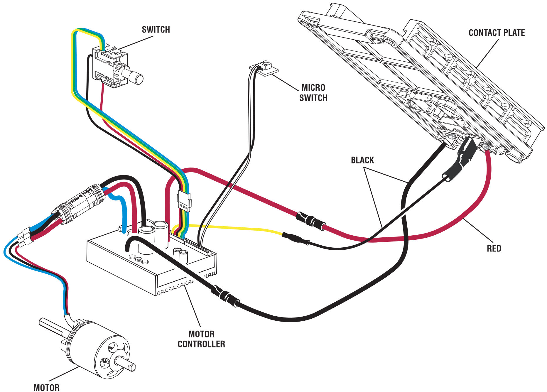
WIRING DIAGRAM
