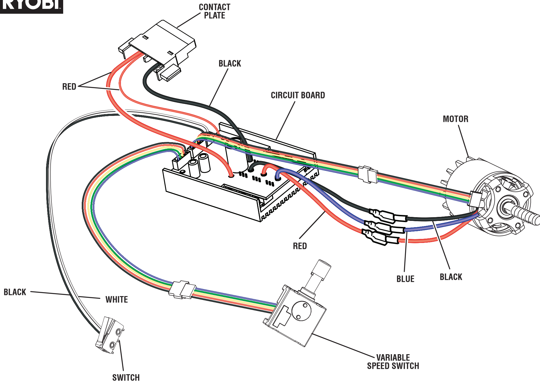
WIRING DIAGRAM
