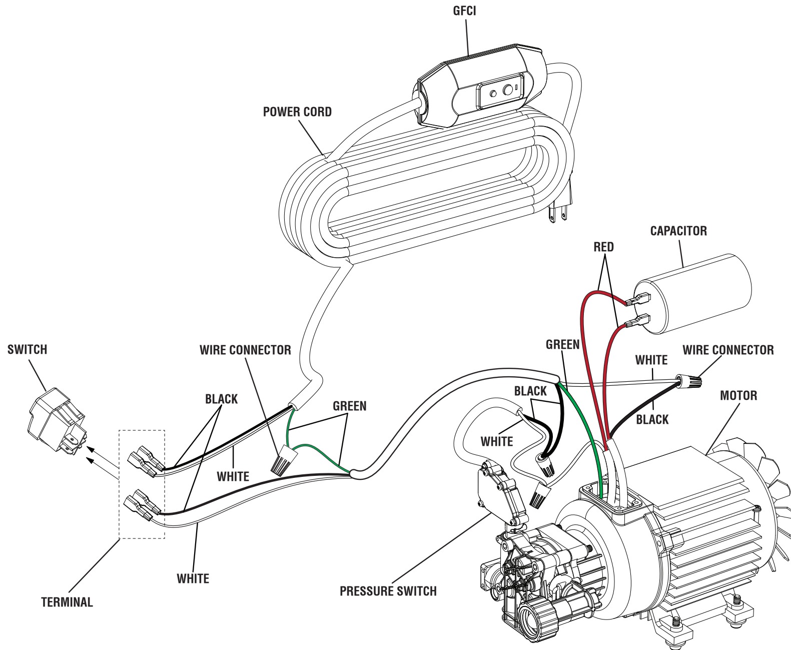
WIRING DIAGRAM
