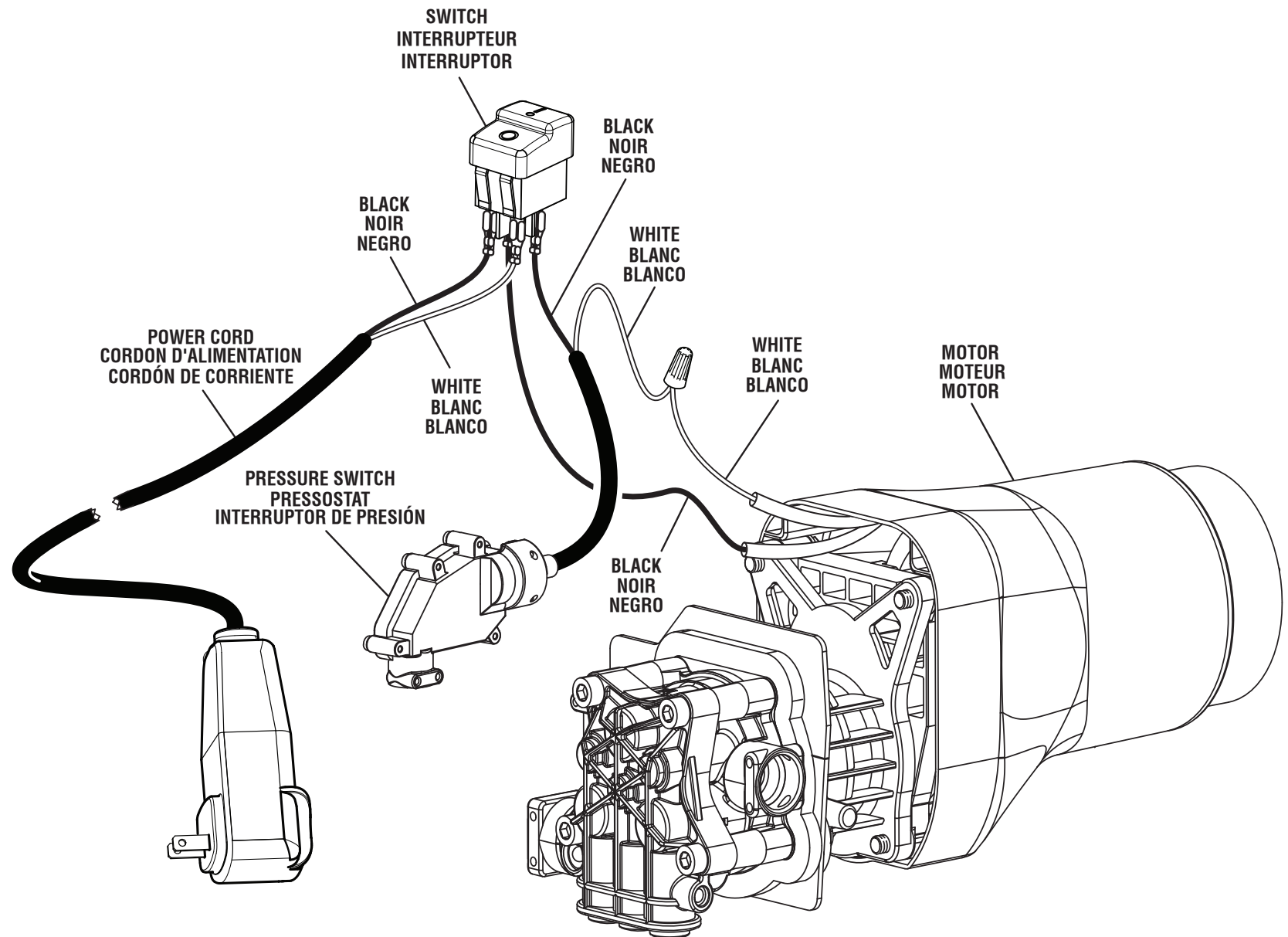
WIRING DIAGRAM
