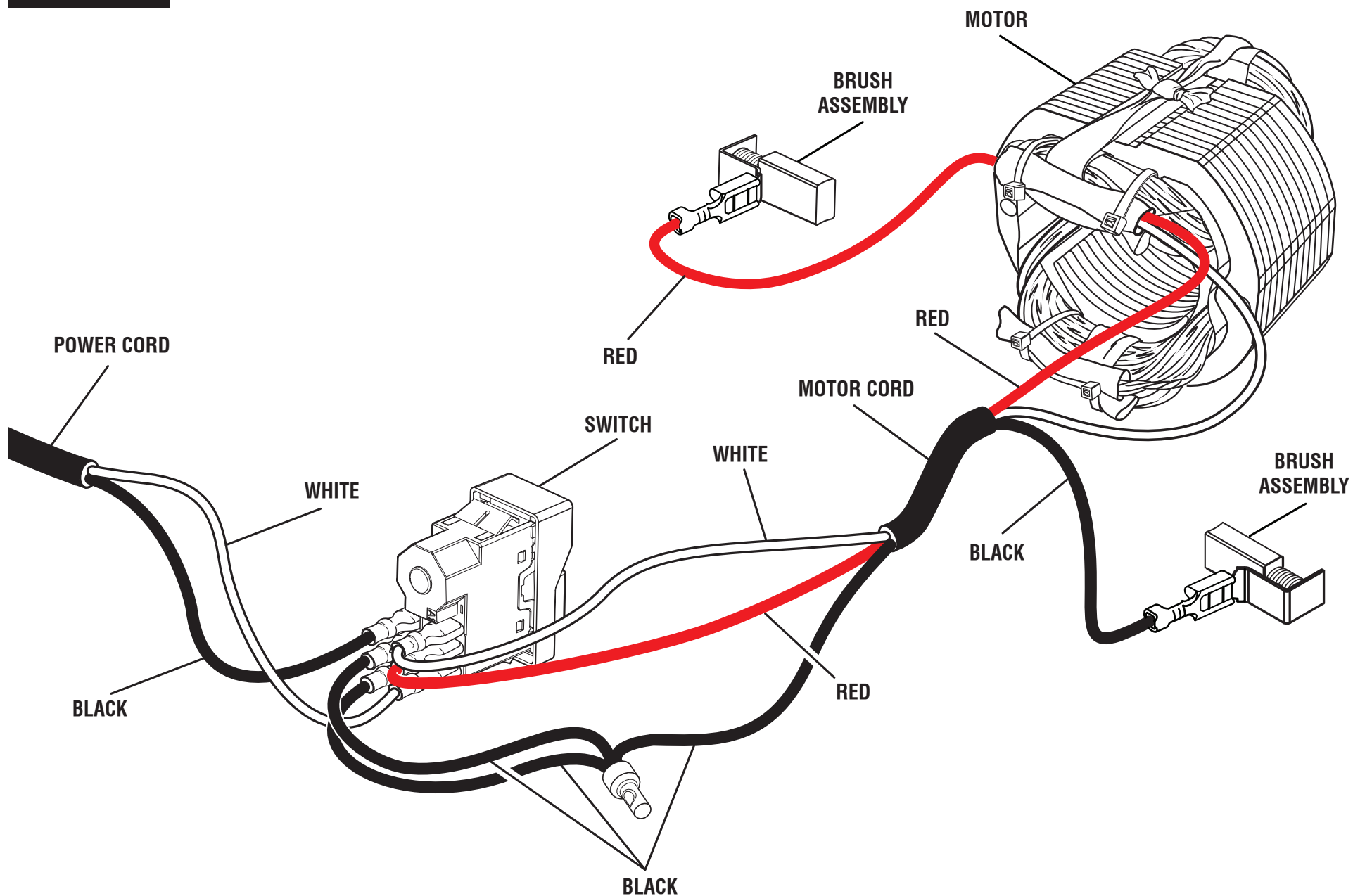
WIRING DIAGRAM
