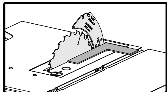
HORIZONTAL ADJUSTMENT
