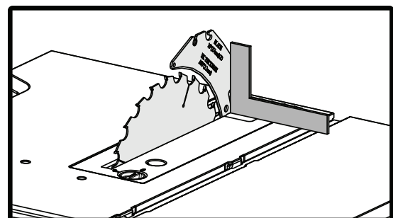
VERTICAL ADJUSTMENT
