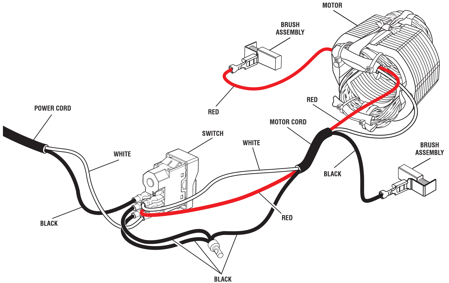
WIRING DIAGRAM
