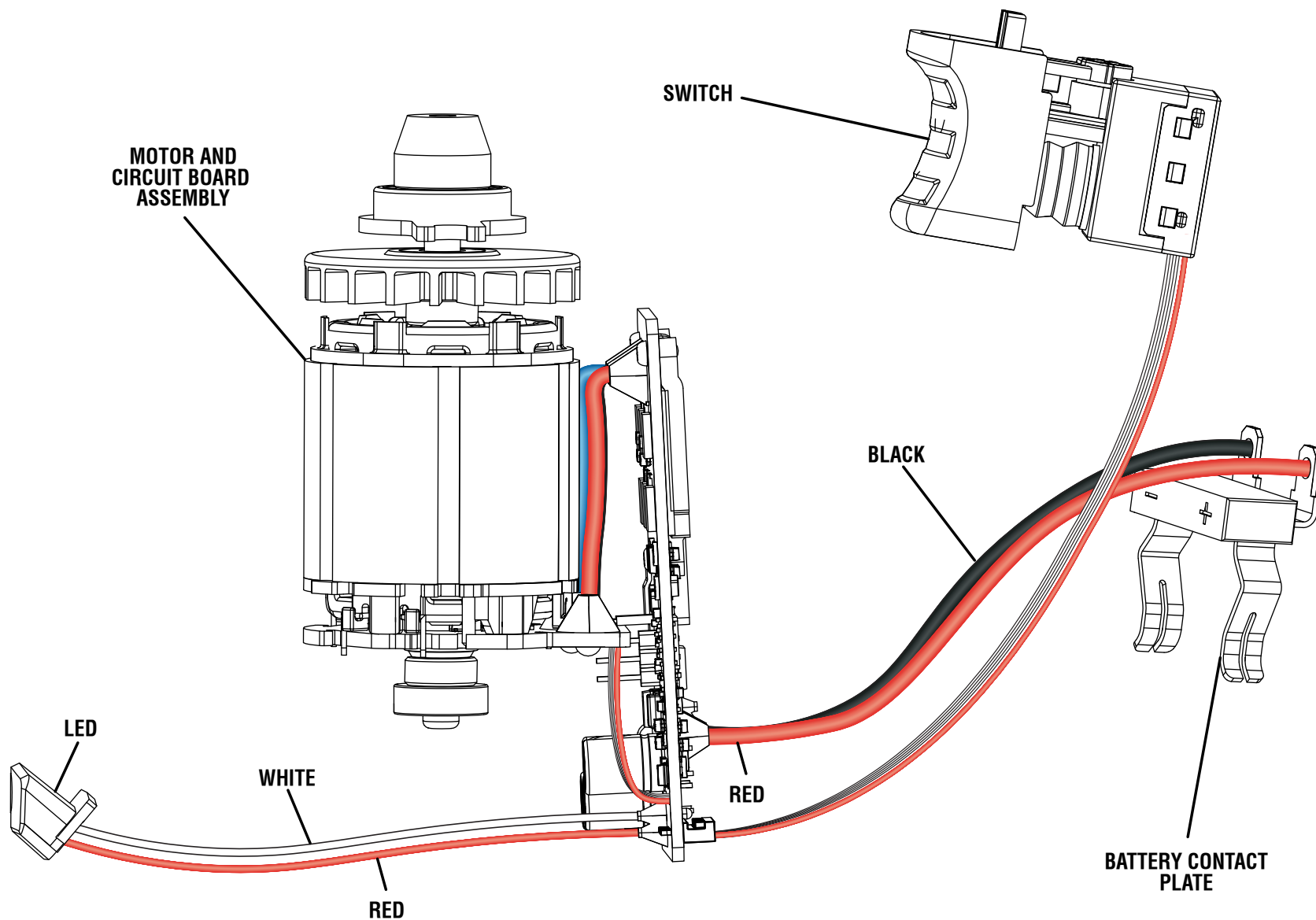
WIRING DIAGRAM
