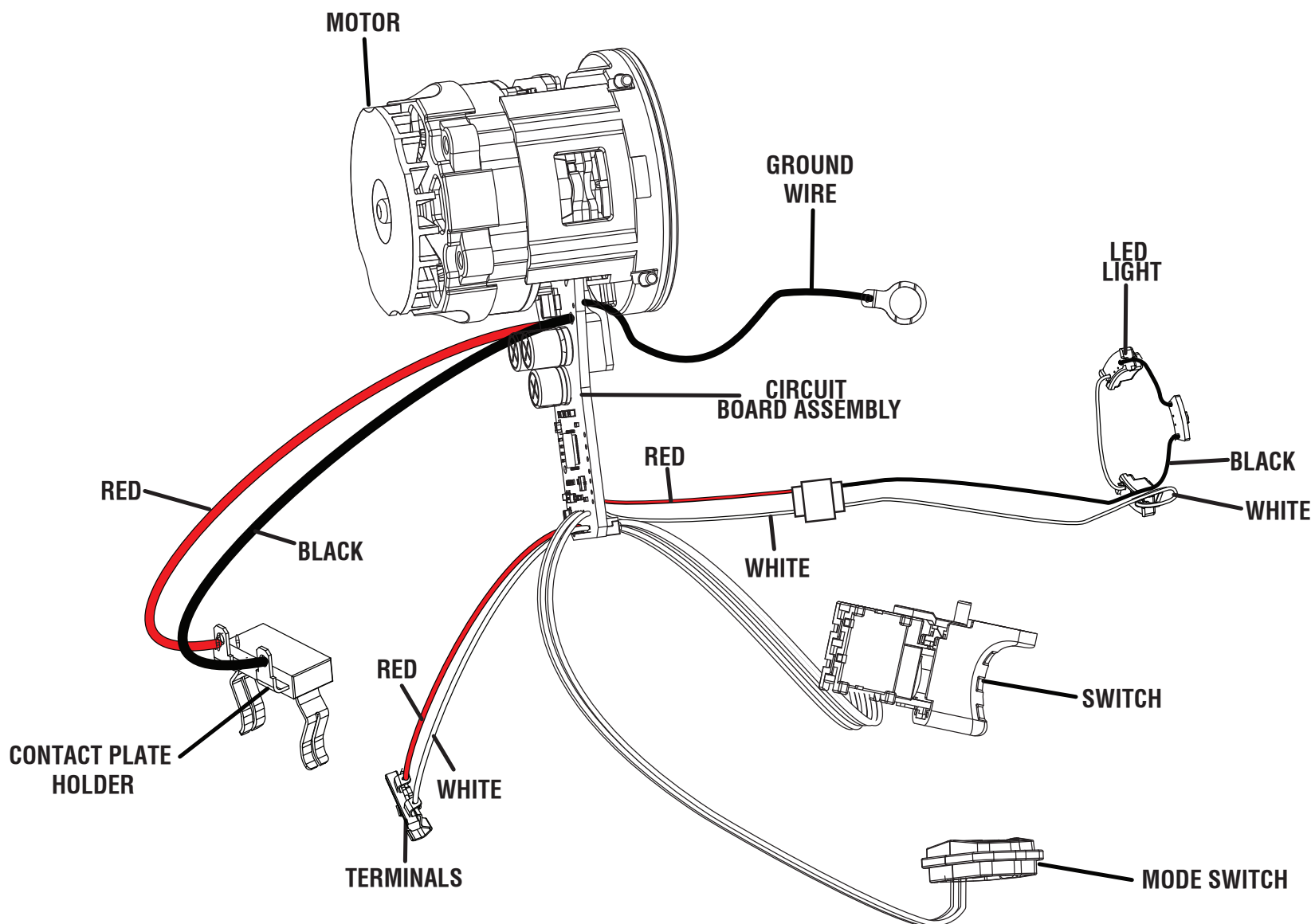
WIRING DIAGRAM
