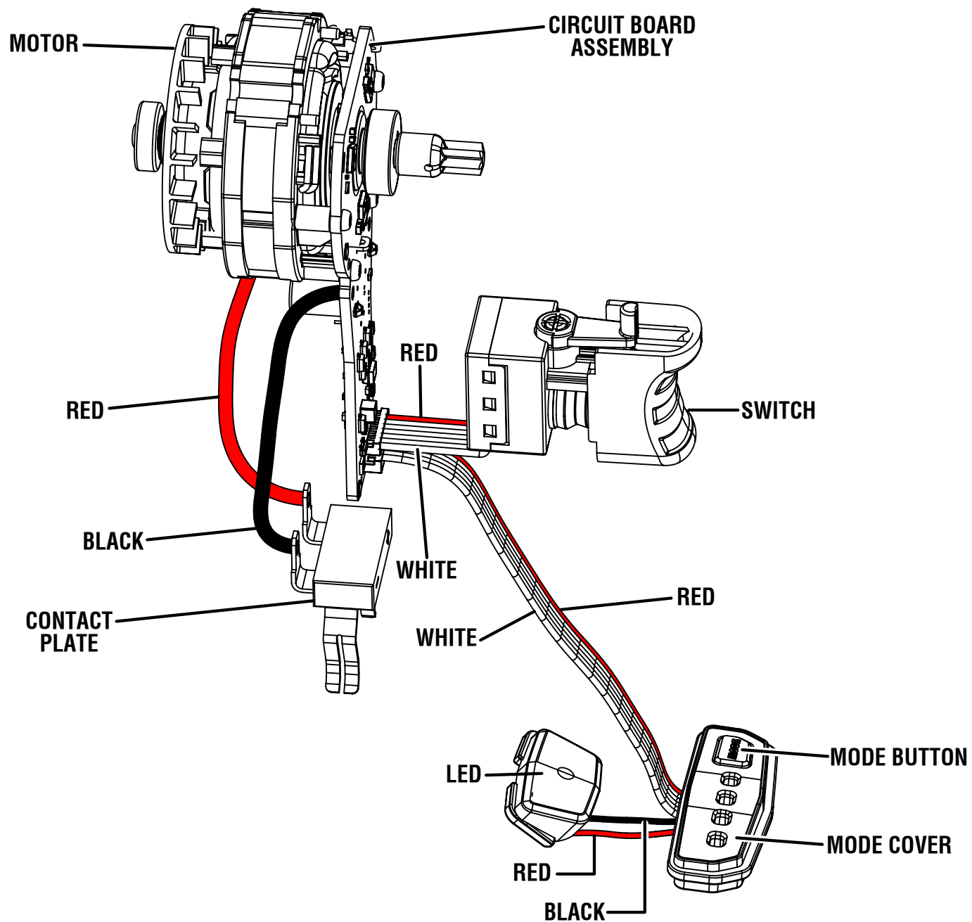
WIRING DIAGRAM
