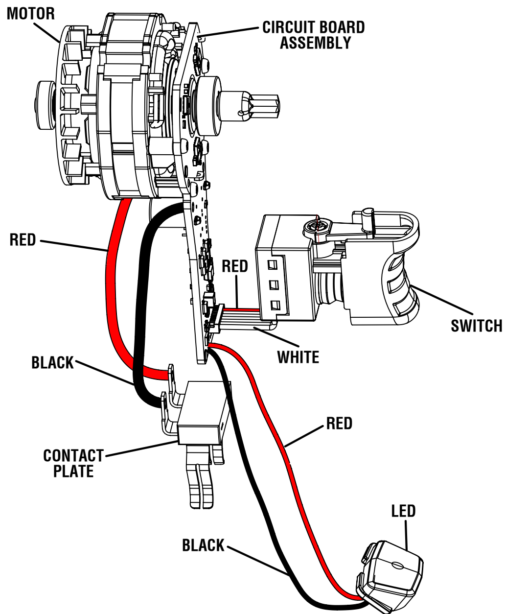
WIRING DIAGRAM
