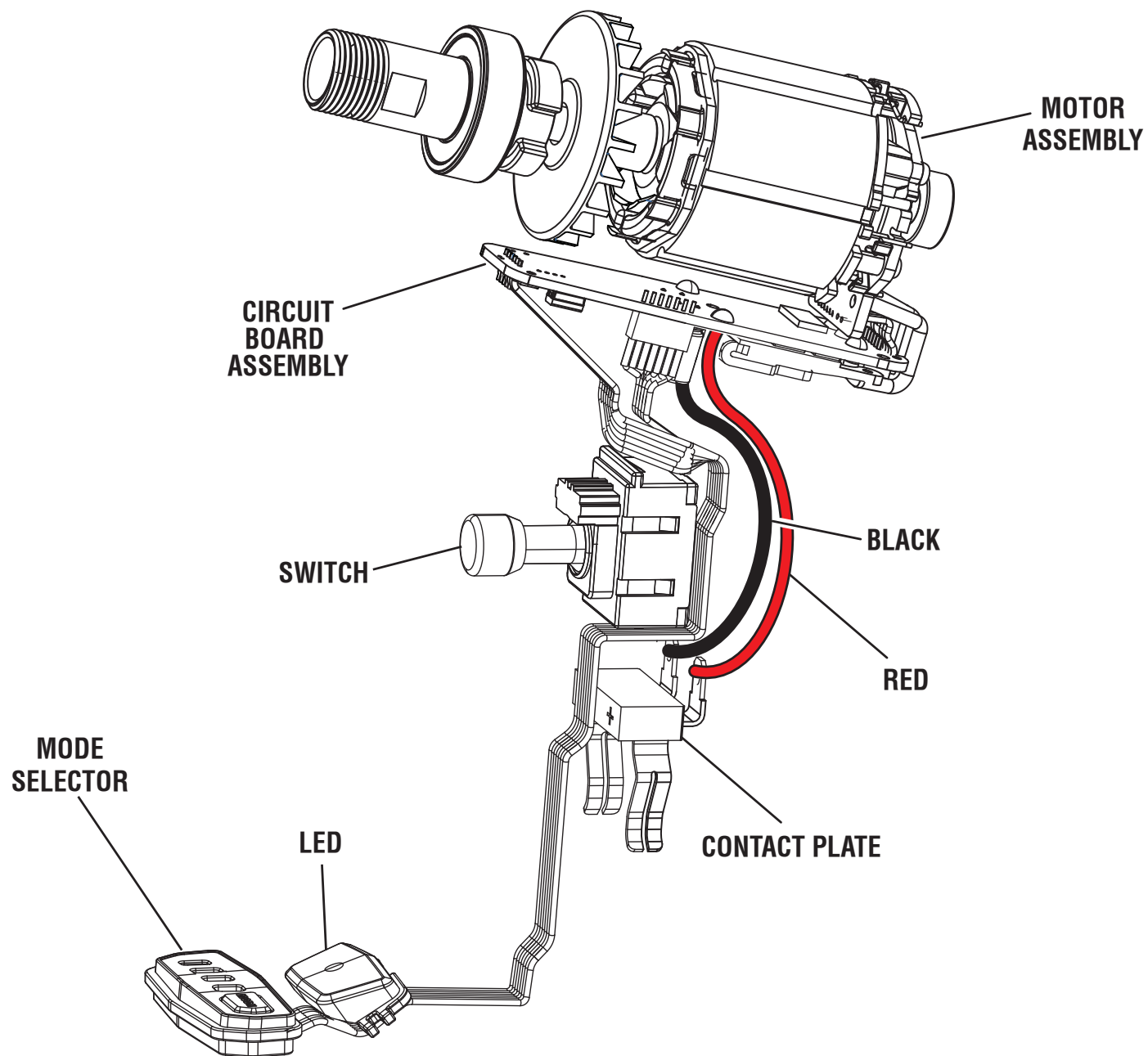
WIRING DIAGRAM
