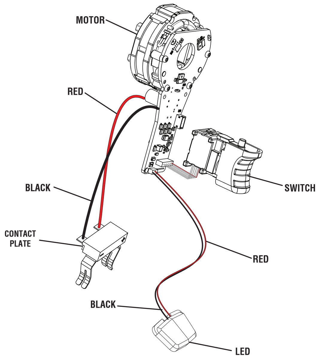
WIRING DIAGRAM
