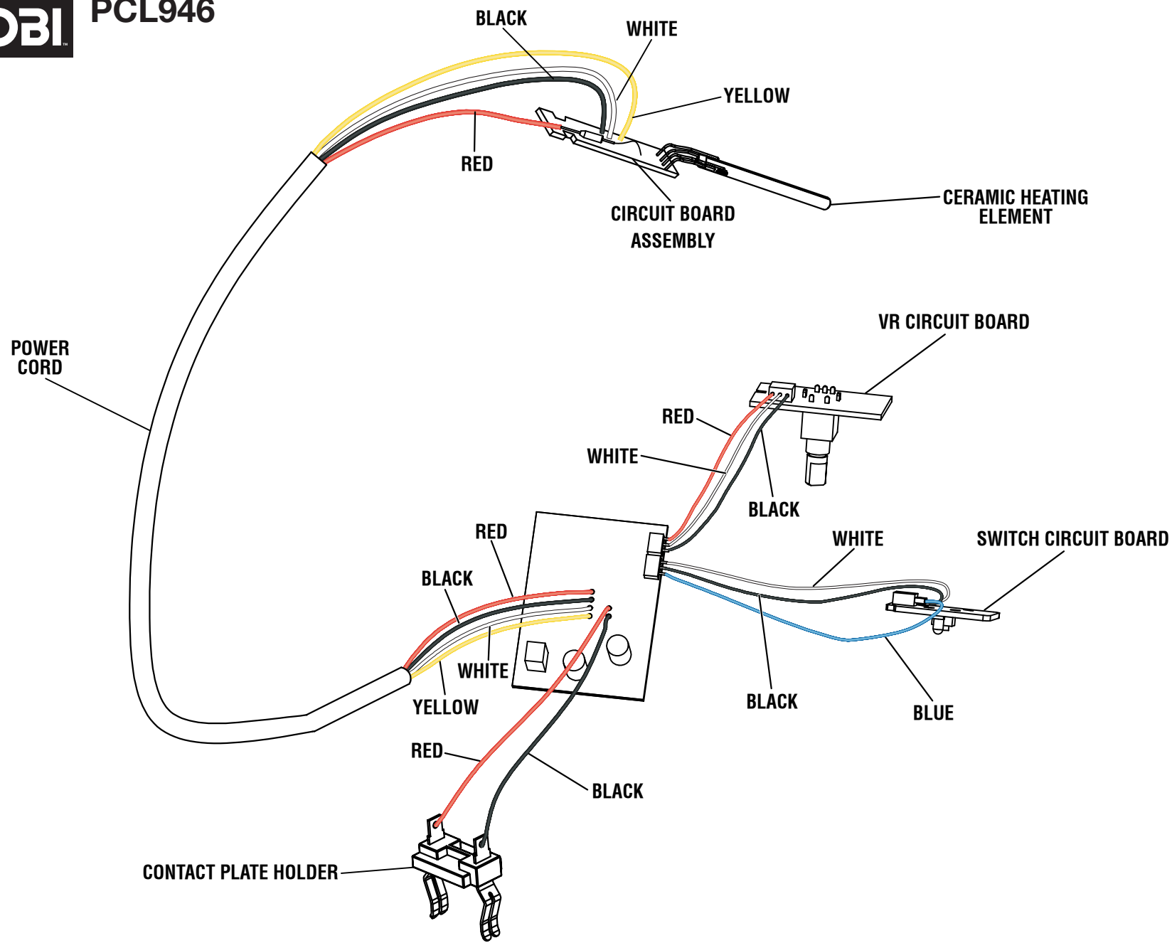
WIRING DIAGRAM
