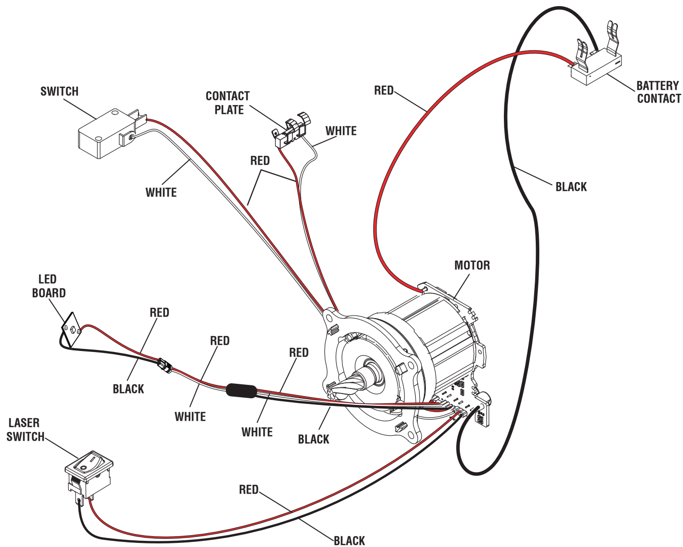
WIRING DIAGRAM
