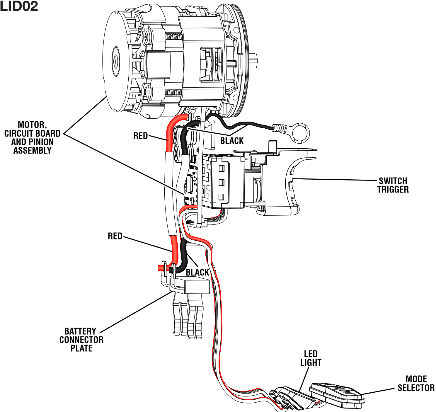
WIRING DIAGRAM
