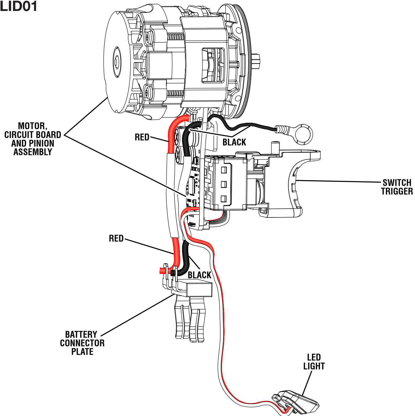
WIRING DIAGRAM
