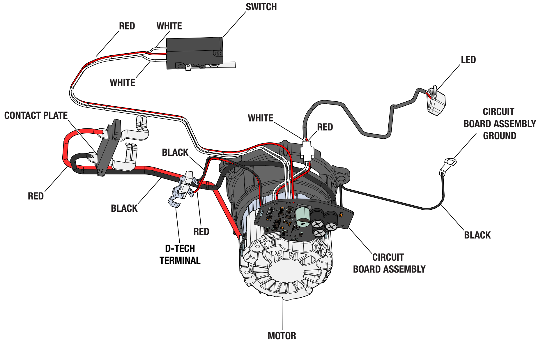
WIRING DIAGRAM
