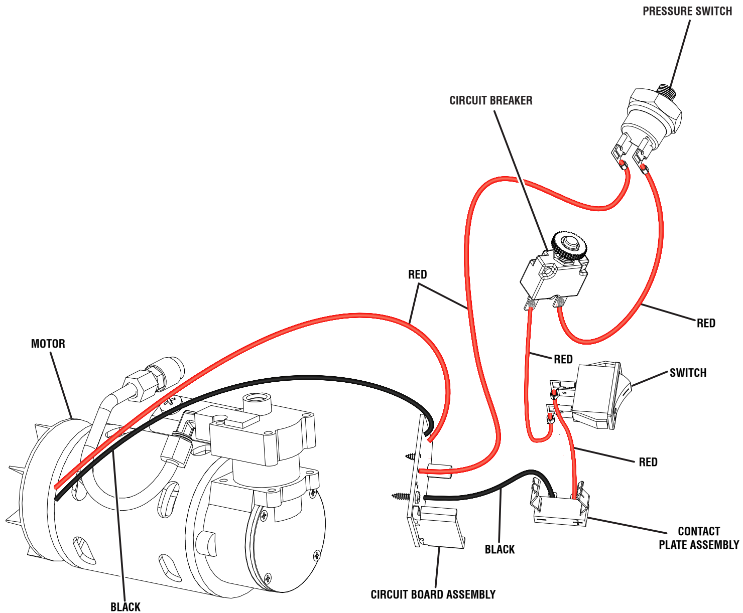
WIRING DIAGRAM
