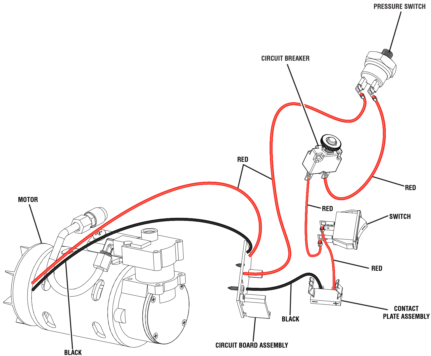
WIRING DIAGRAM
