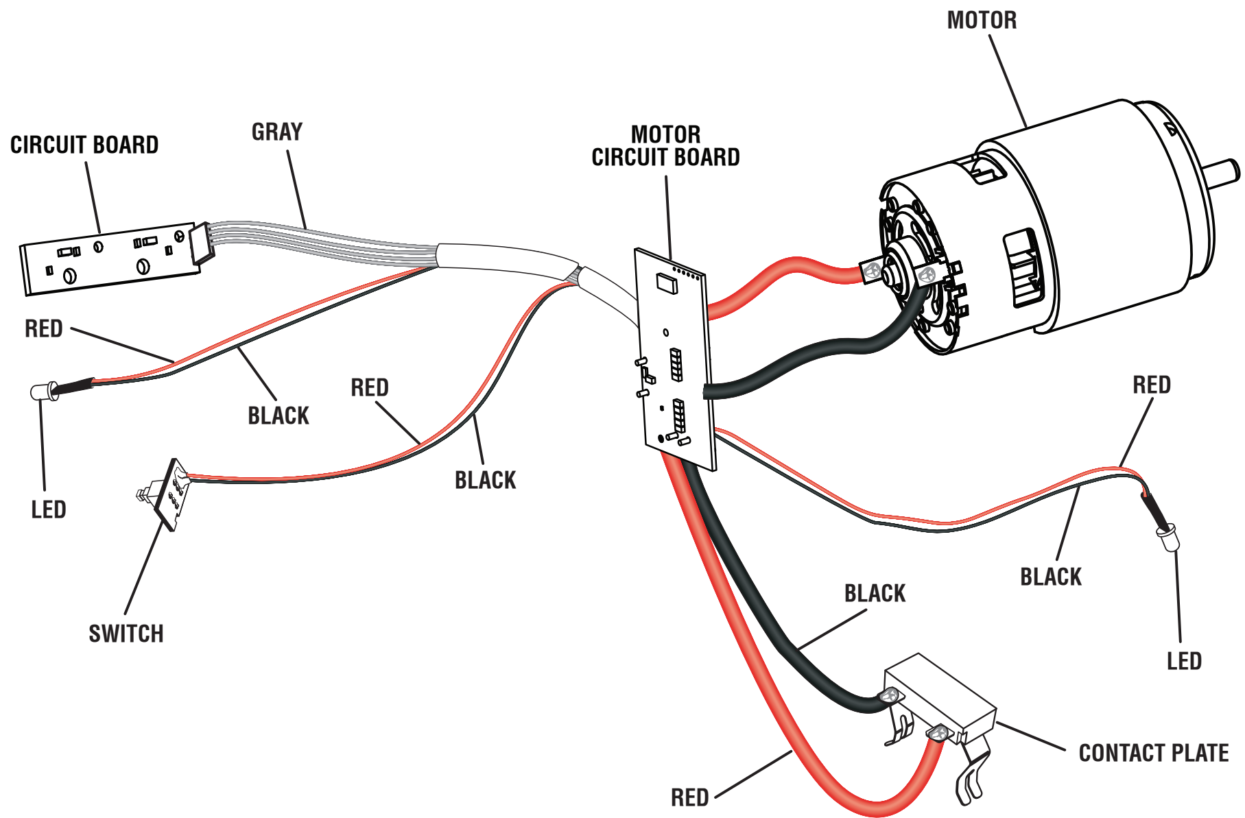
WIRING DIAGRAM
