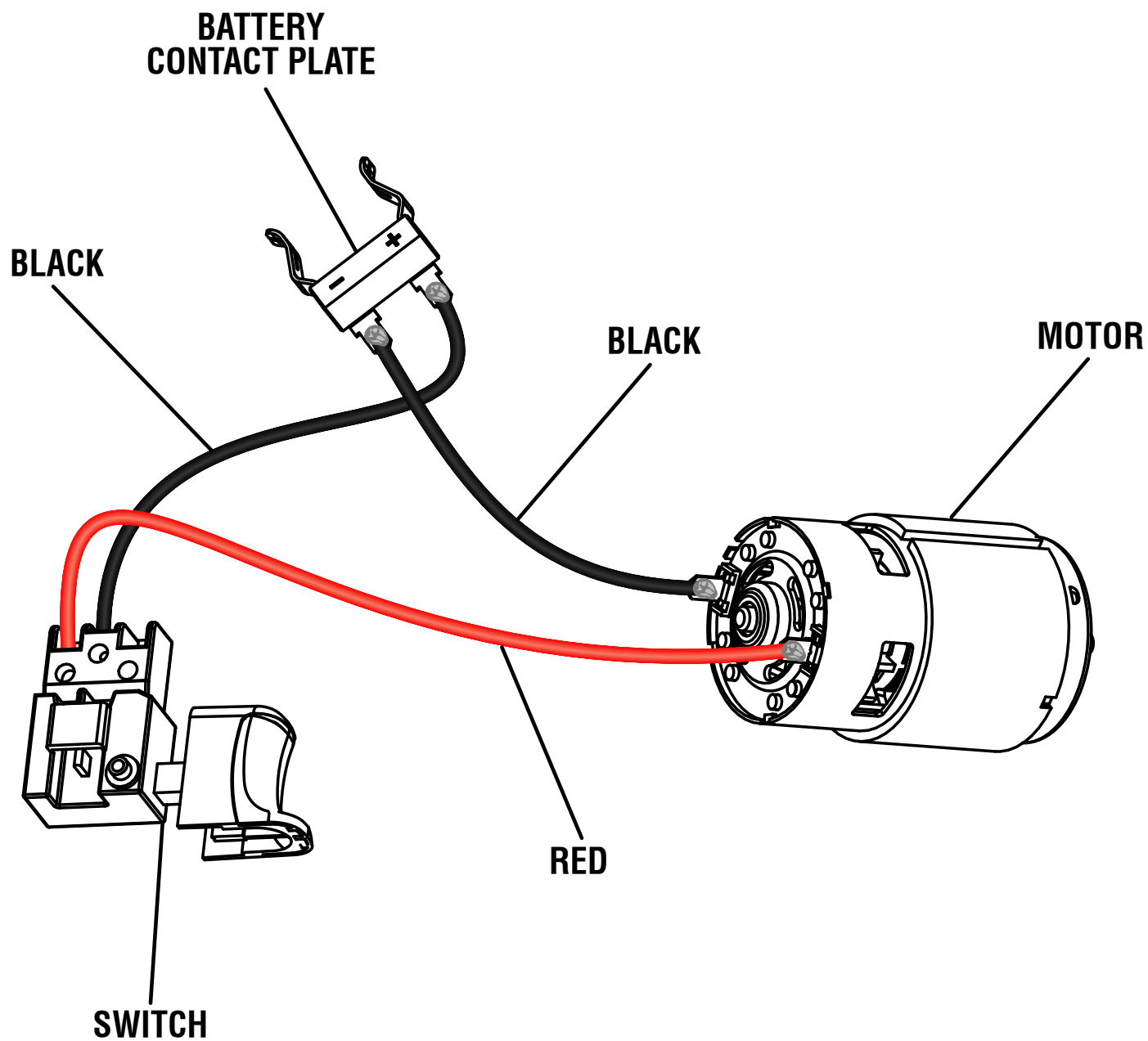
WIRING DIAGRAM
