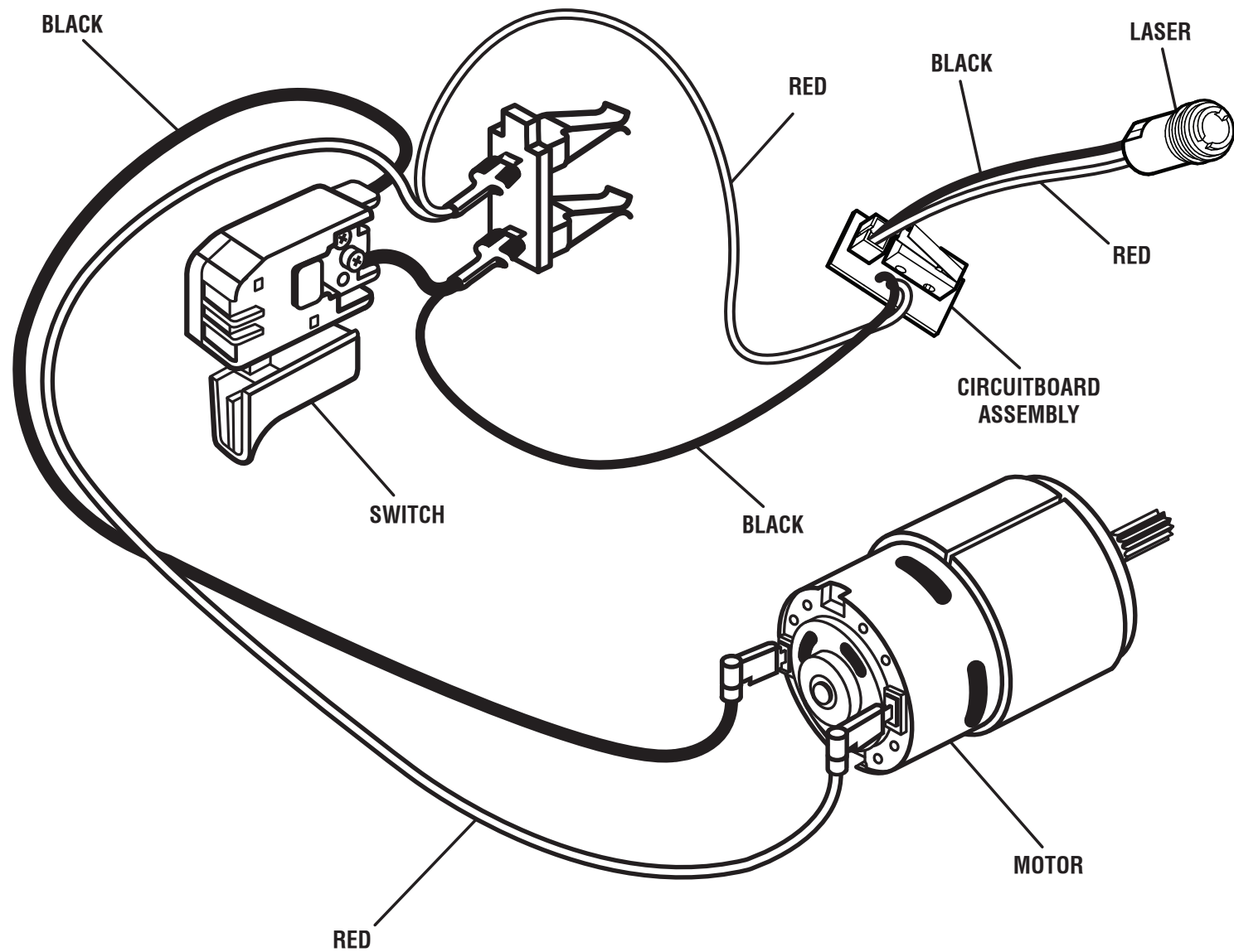
WIRING DIAGRAM
