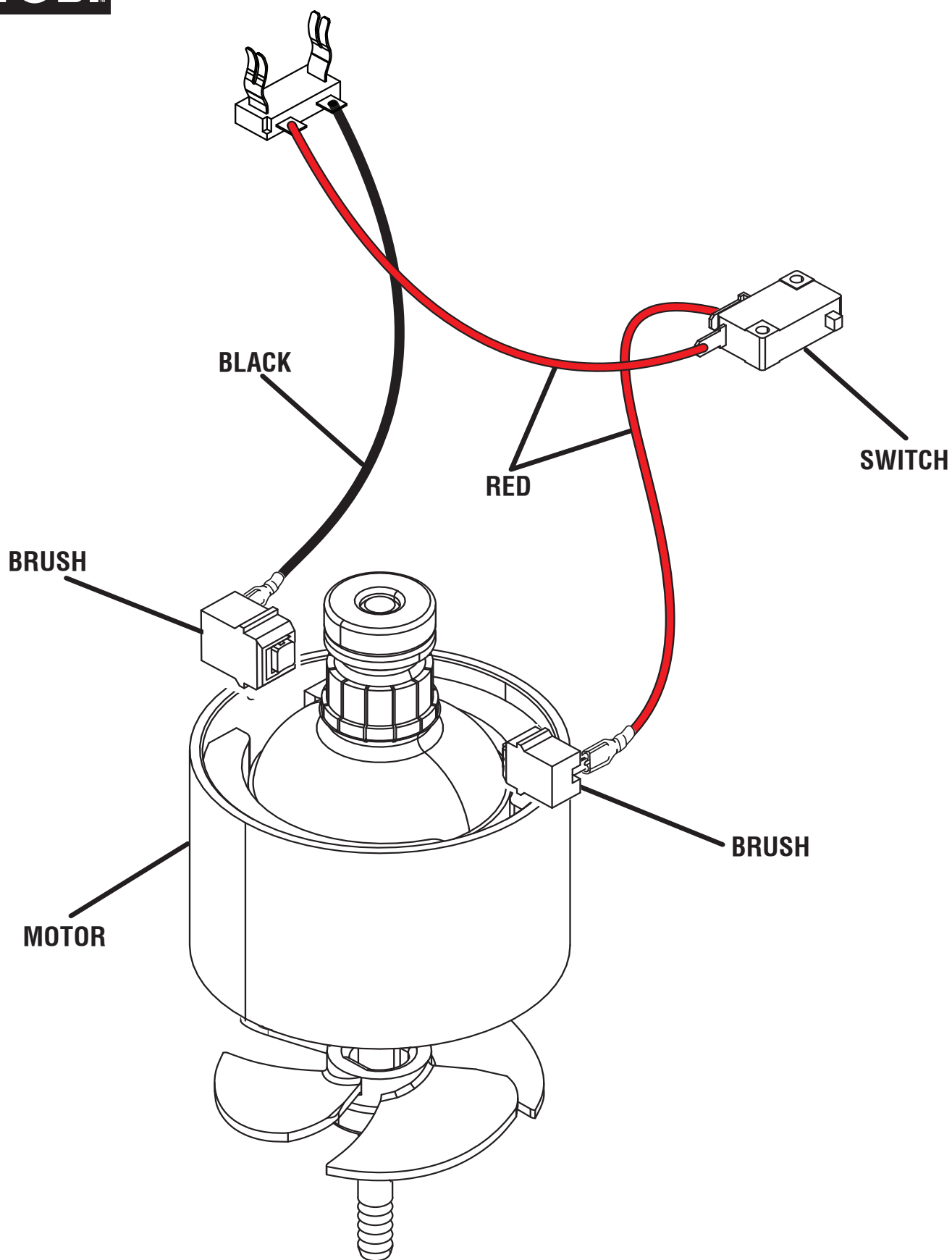
WIRING DIAGRAM
