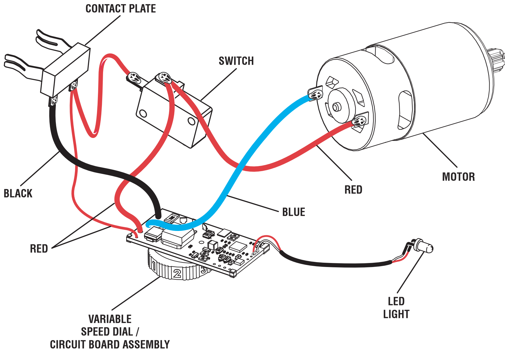
WIRING DIAGRAM
