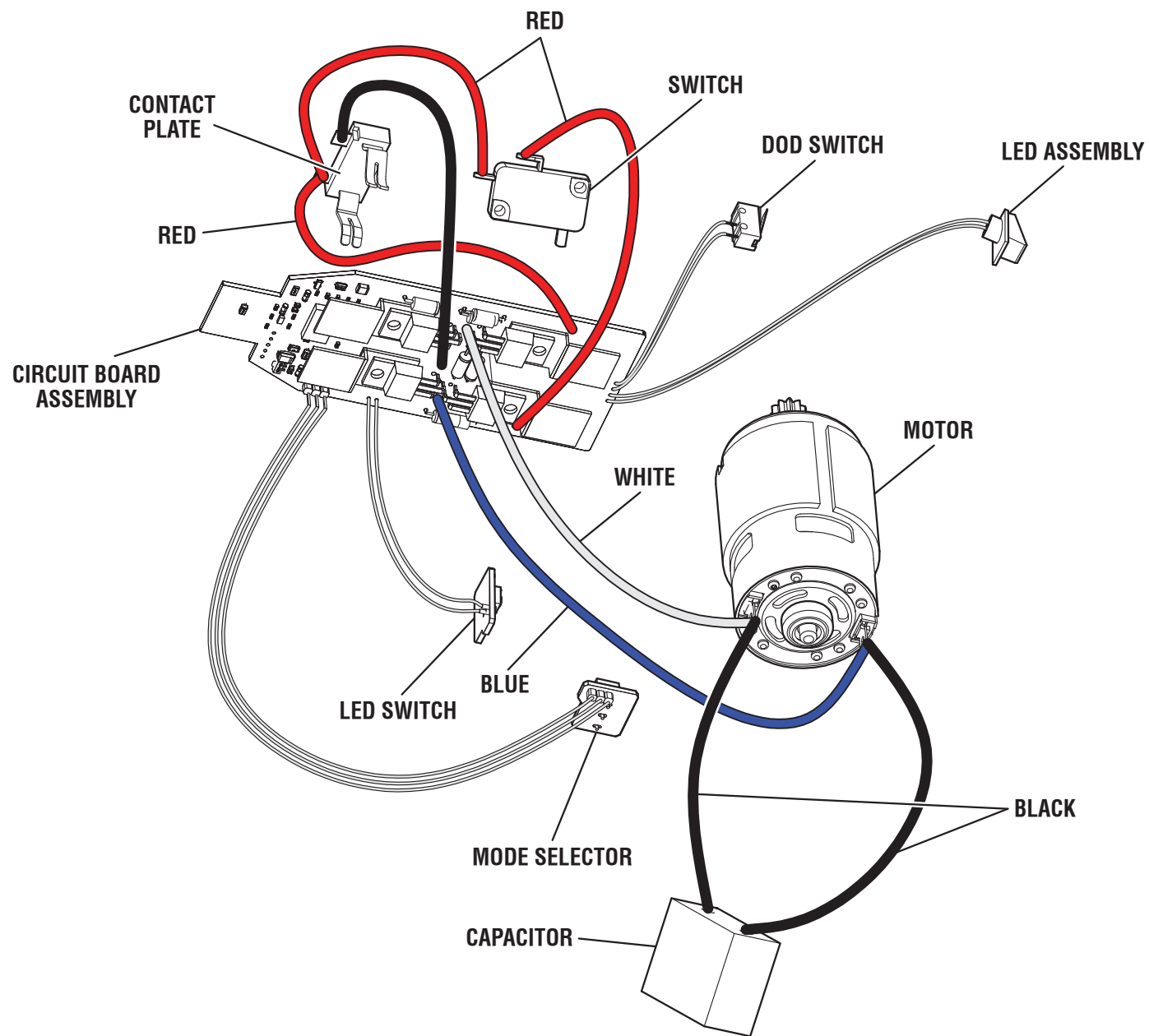
WIRING DIAGRAM
