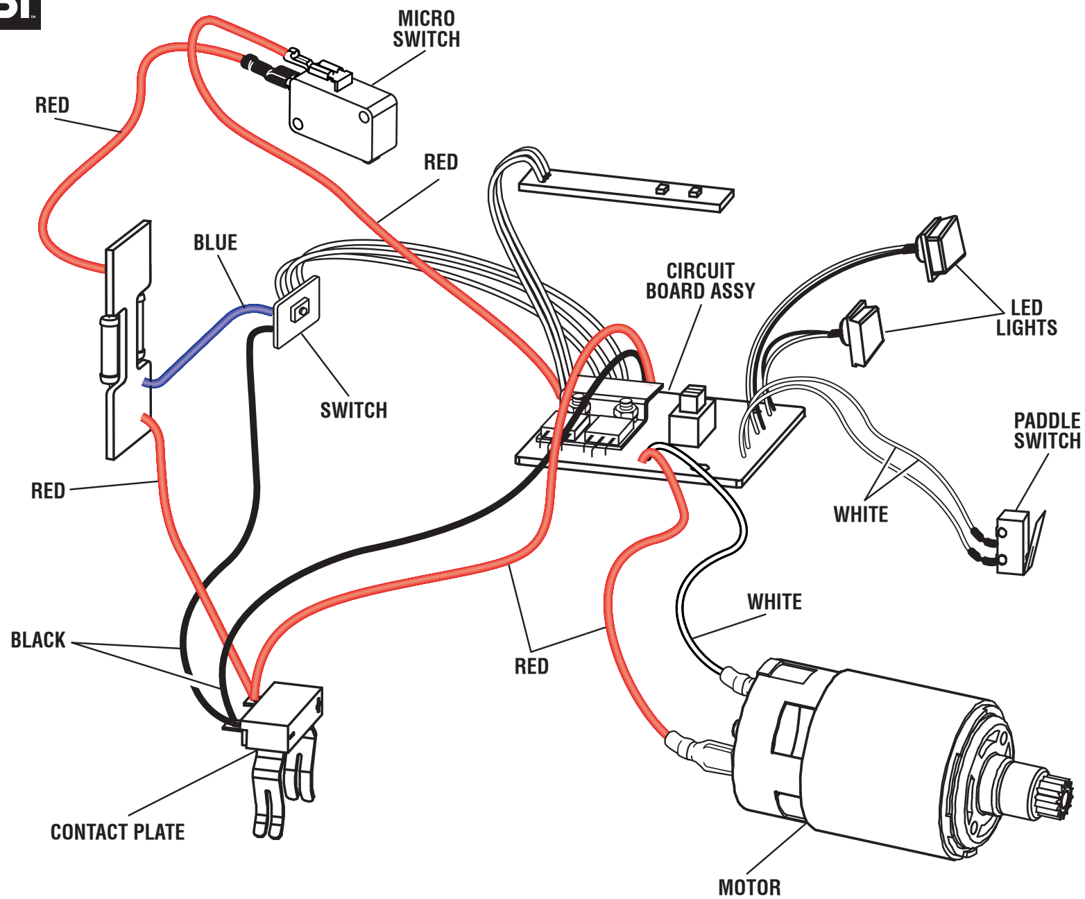
WIRING DIAGRAM
