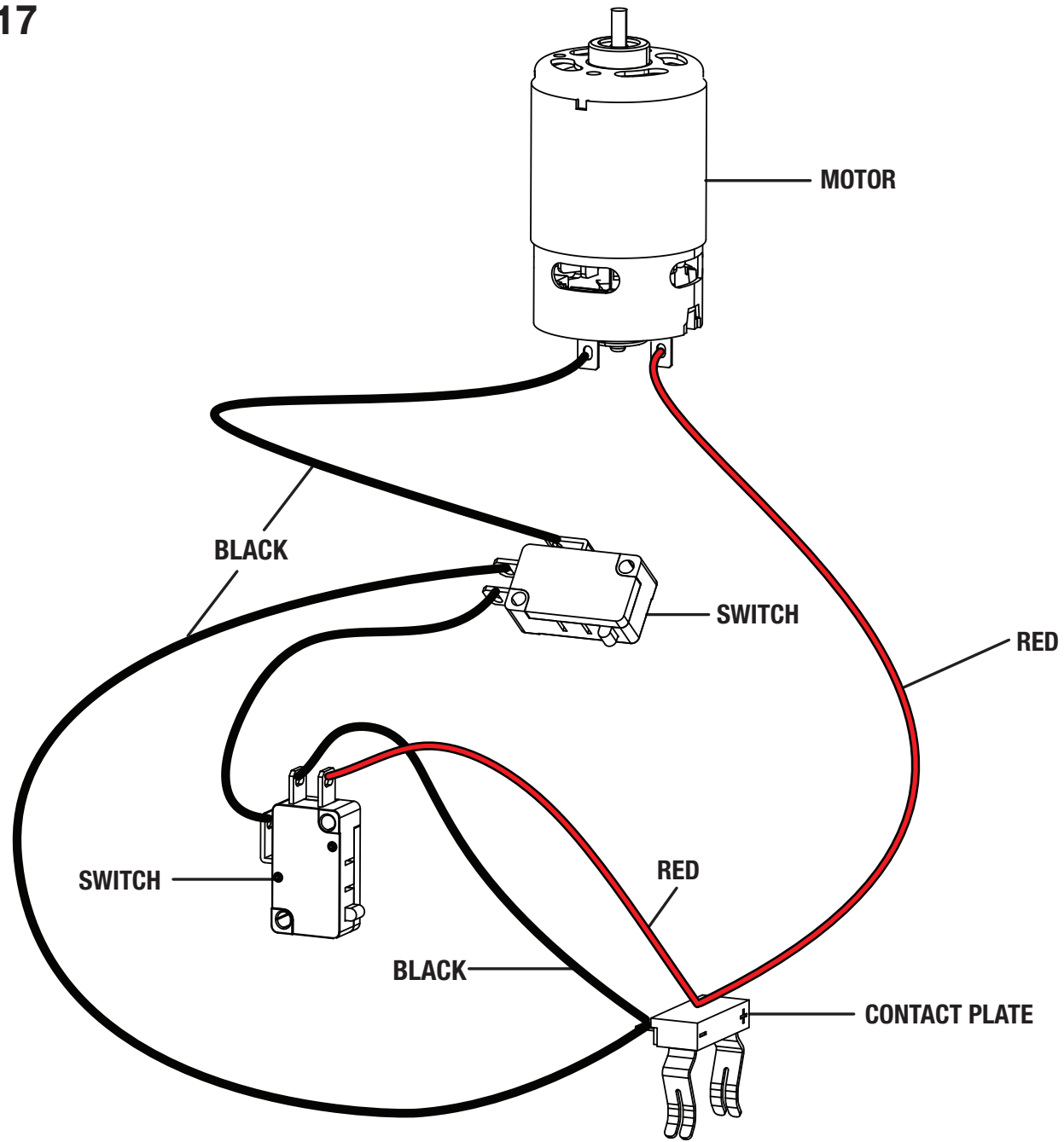
WIRING DIAGRAM
