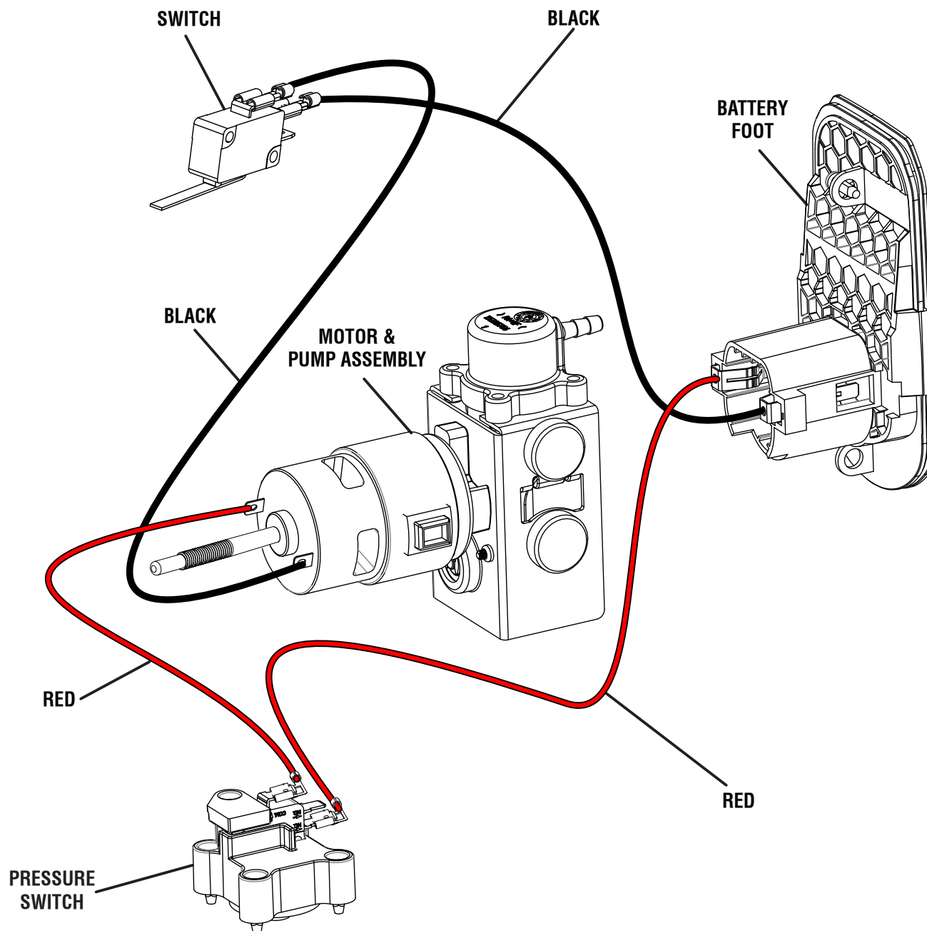
WIRING DIAGRAM
