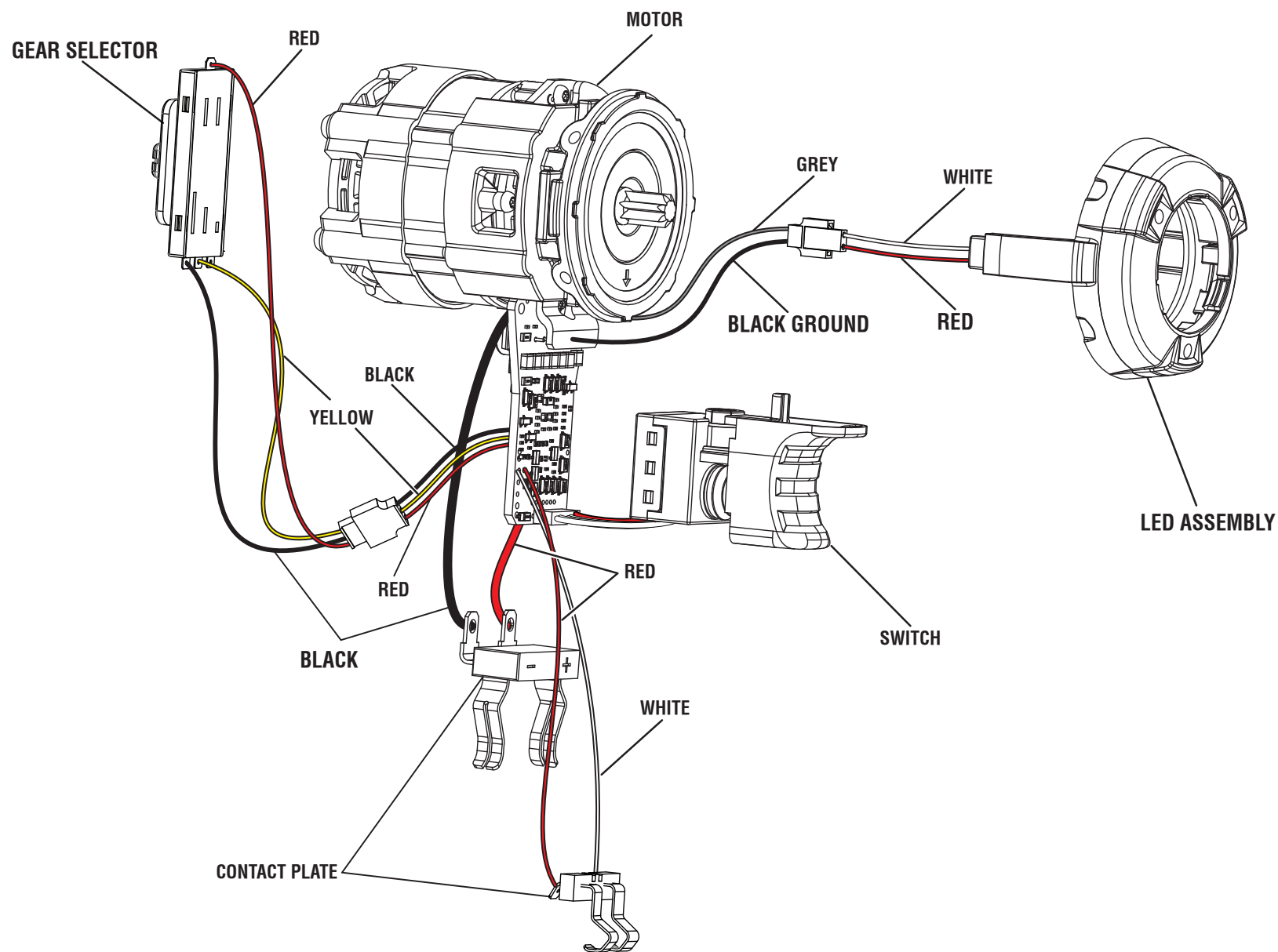
WIRING DIAGRAM
