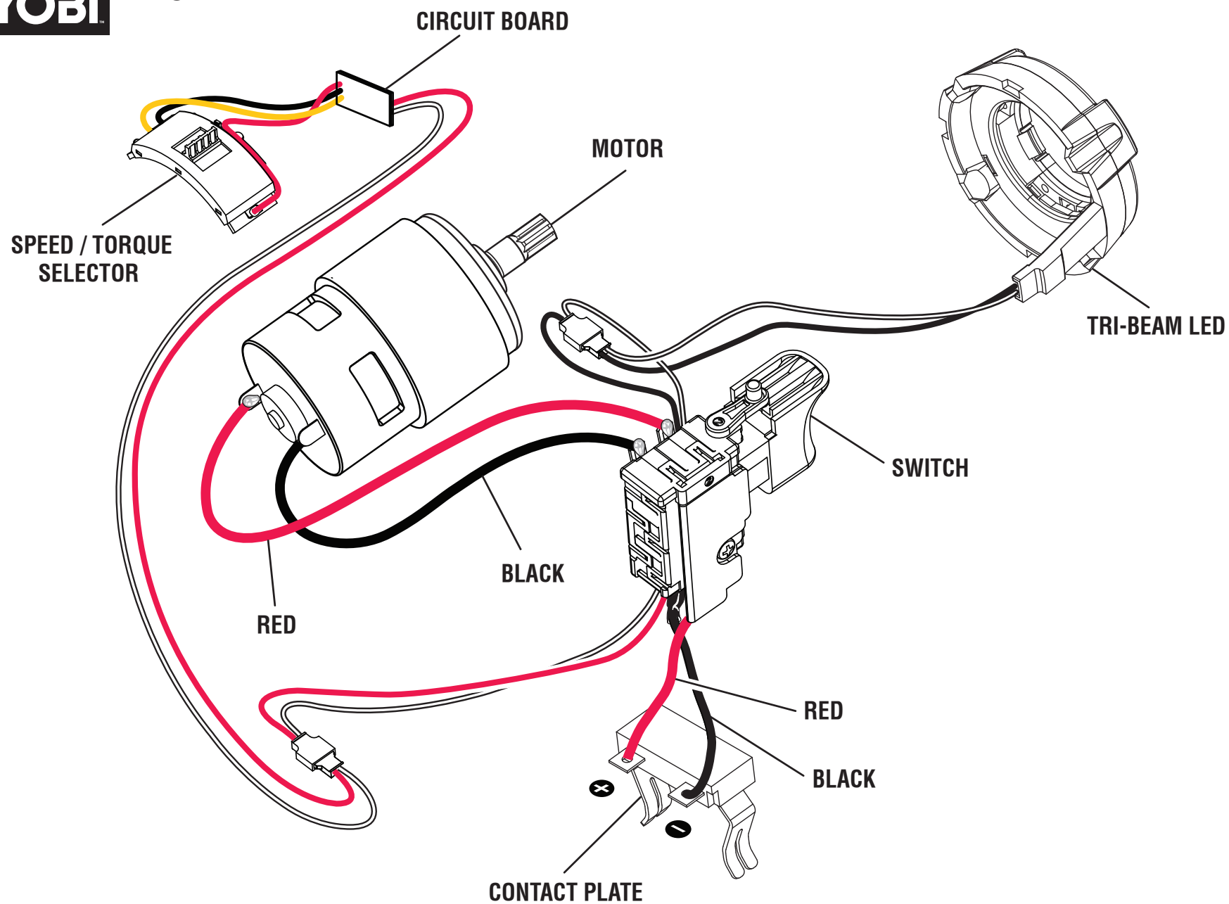
WIRING DIAGRAM
