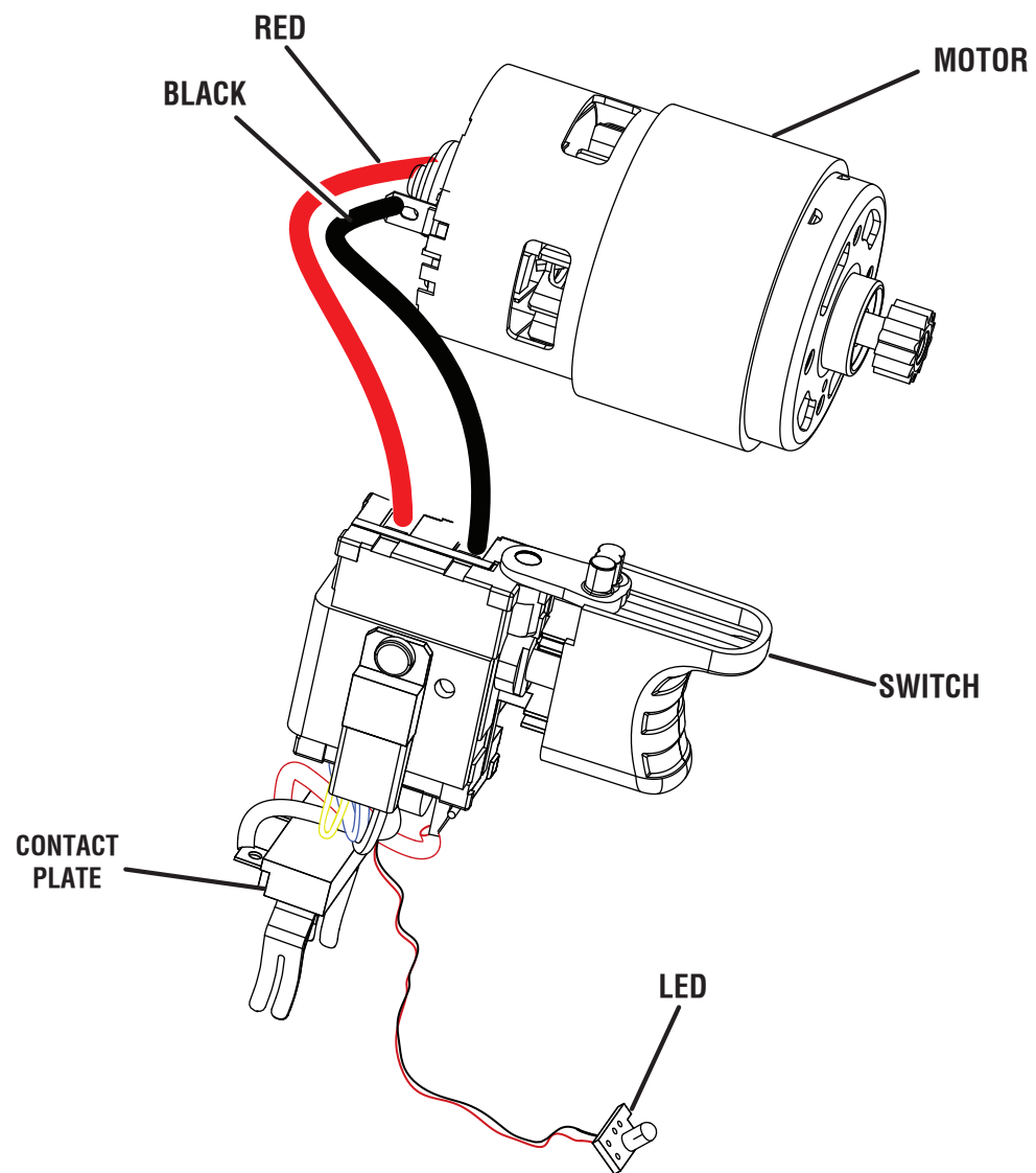
WIRING DIAGRAM
