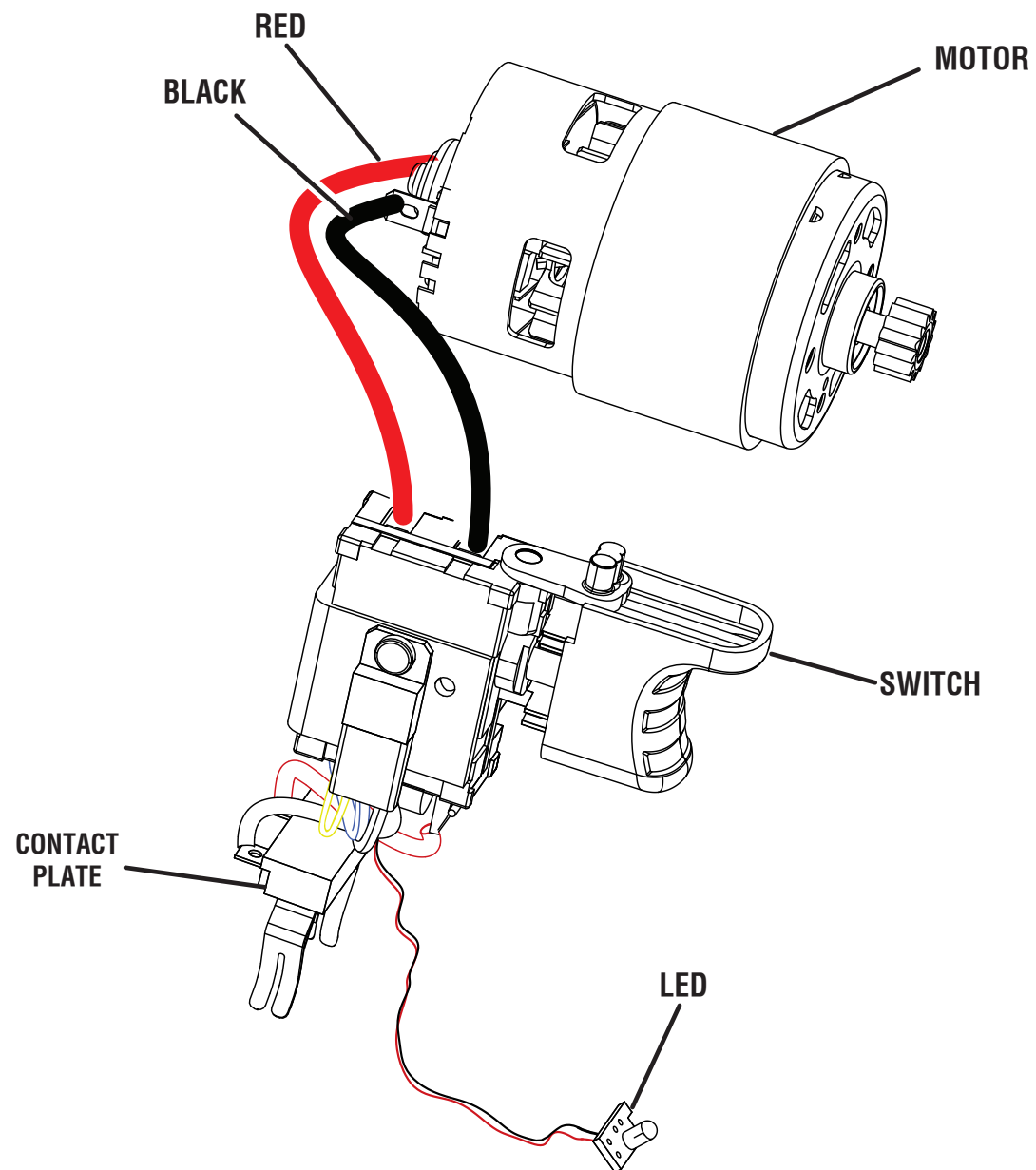
WIRING DIAGRAM
