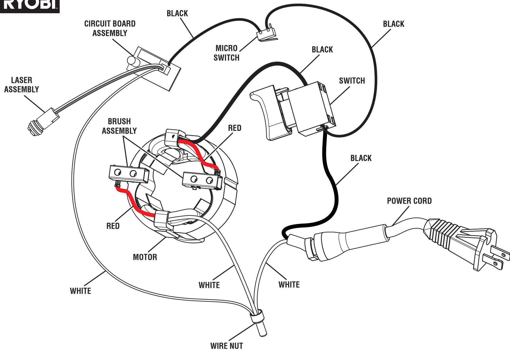
WIRING DIAGRAM
