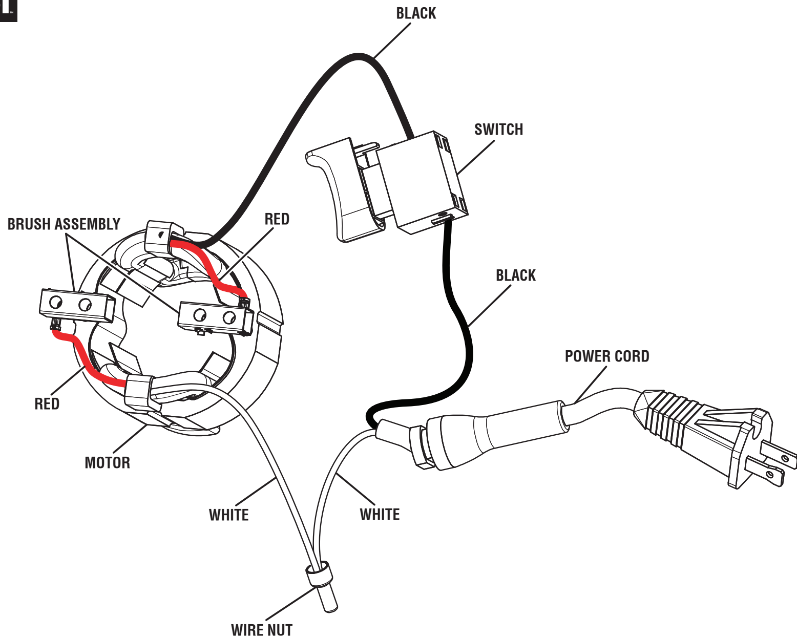
WIRING DIAGRAM
